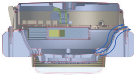
Figure 1, Heat removal illustration for an integral LED luminaire
