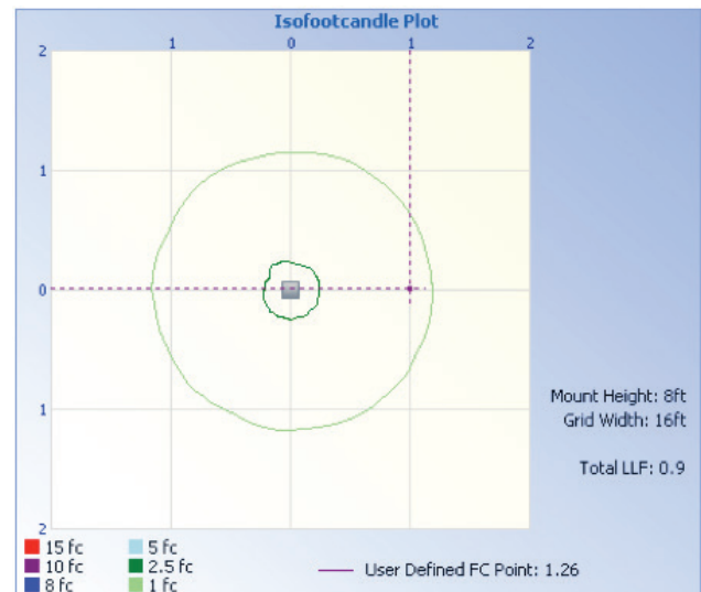
Figure 7 Plot with LED Retrofit Lamp
