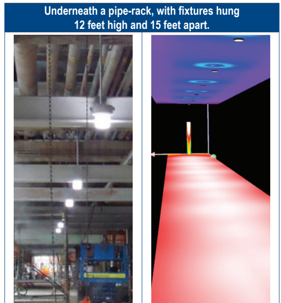
Figure 13 Pipe-rack Application with a 48W (150W equivalent) Mercmaster LED Low Profile Luminaire with Refractor Replaced with Diffused Polycarbonate Globe
